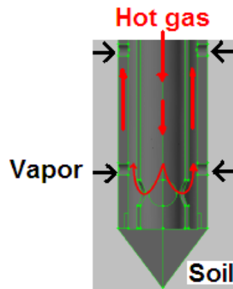
Fig 5. Heating pipe
