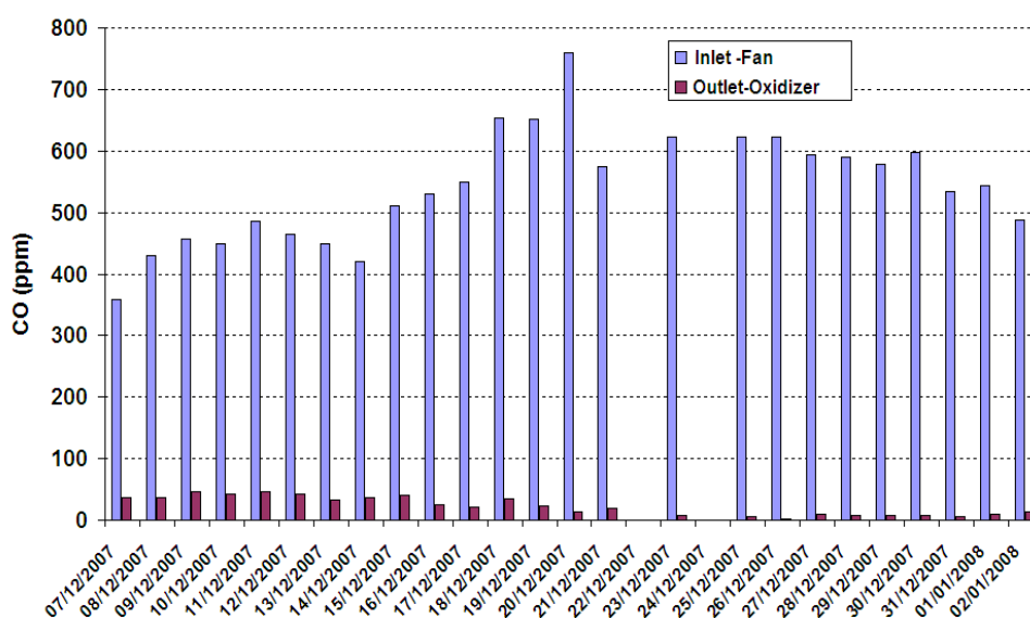
Fig 9. Evolution of carbon monoxide concentration.
