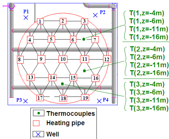
Fig 7. Soil thermocouples location
