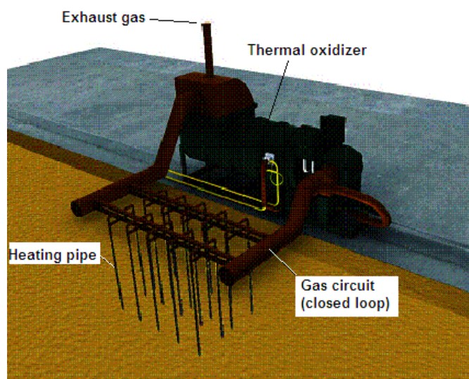
Fig 1. Thermopile© in-situ system
