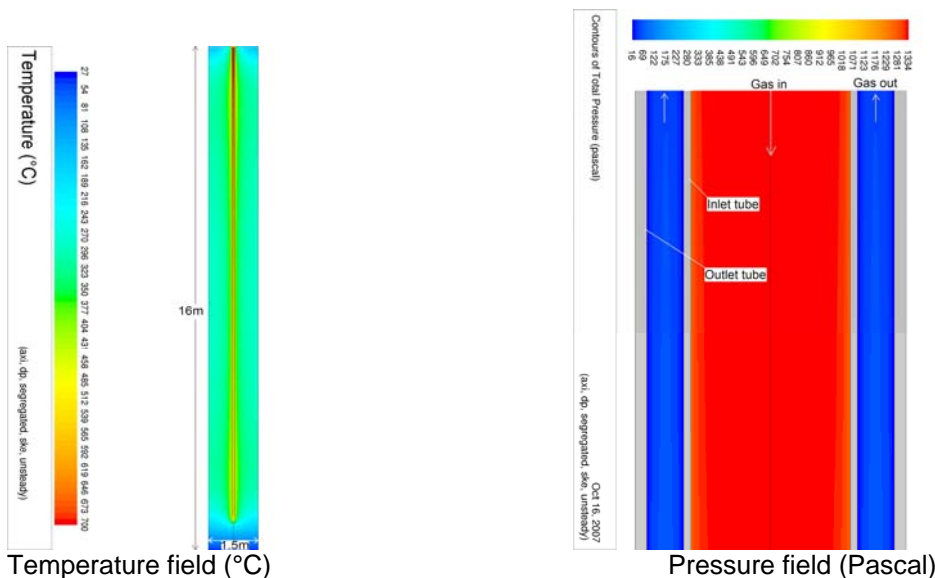
Fig 6. Temperature and pressure fields.
