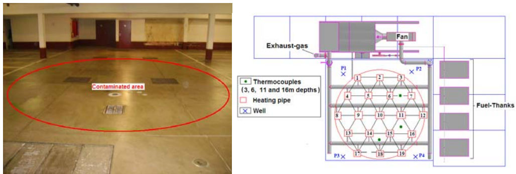
Fig 3. Contaminated area and Thermopile© installation
